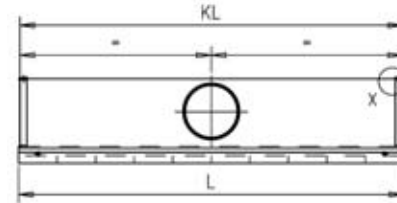
Plenum with 1 connection inlet
