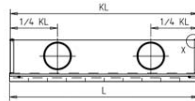
Plenum with 2 connection inlets
