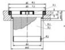
BDA-K / -M / -A with mounting frame (-ER) without flange
