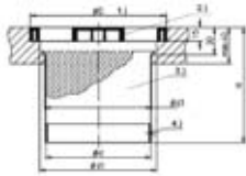
BDA-K / -M / -A without mounting frame
